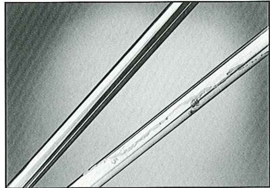
NitroSteel compared to chrome after salt spray testing shows superior corrosion resistance.
